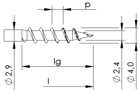
With and without thread variation, with toothed tip
