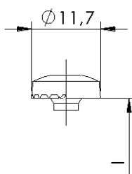
Pan head with and without milling ribs underneath the head
