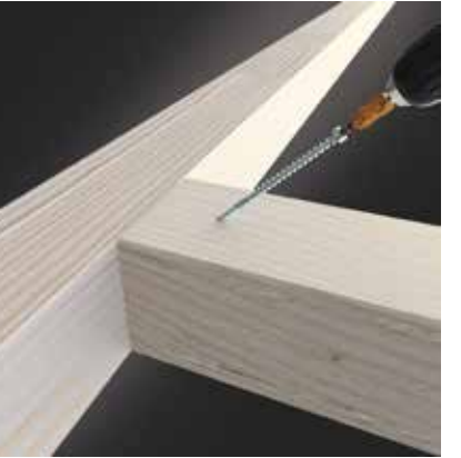
Connection of main and auxiliary beams
